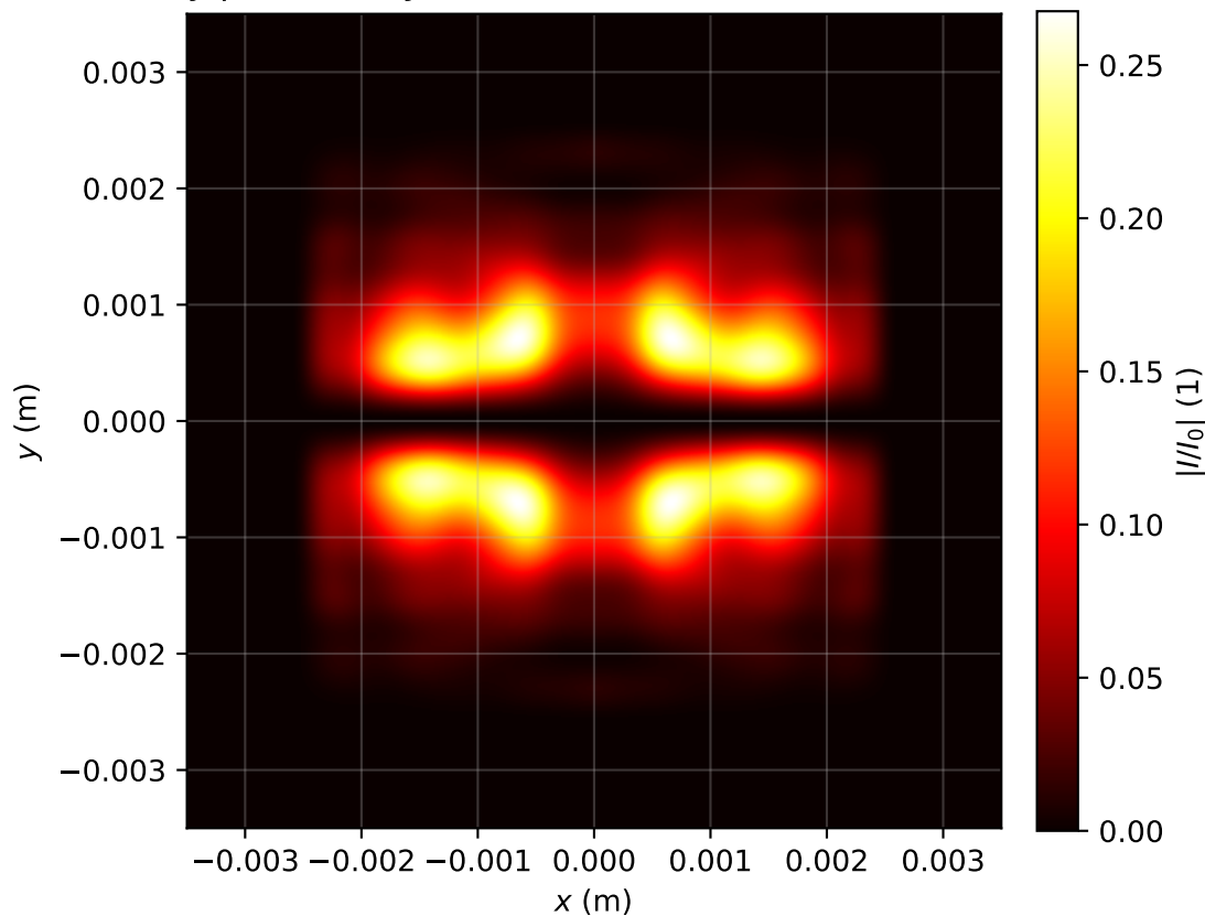
Intensity profile I(x, y, z = 3.582)/I_0 , P_{in}=4.0P_{cr} , artificial time
